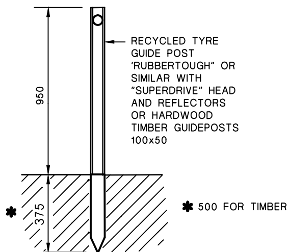
SKETCH C GUIDE POST
