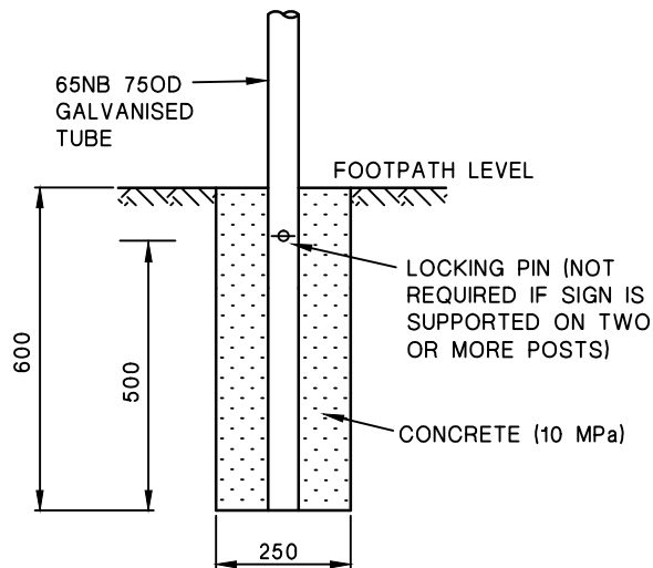
SKETCH A ERECTION OF SIGN IN FOOTWAY AREAS
