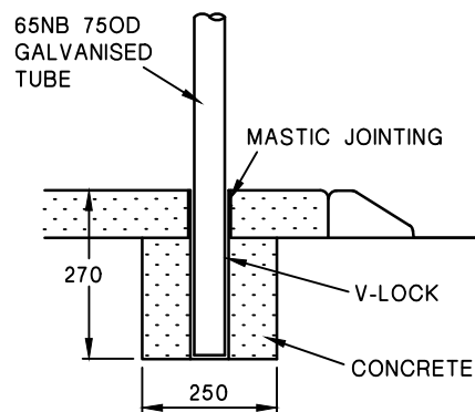
SKETCH D ERECTION OF SIGN IN MEDIANS
